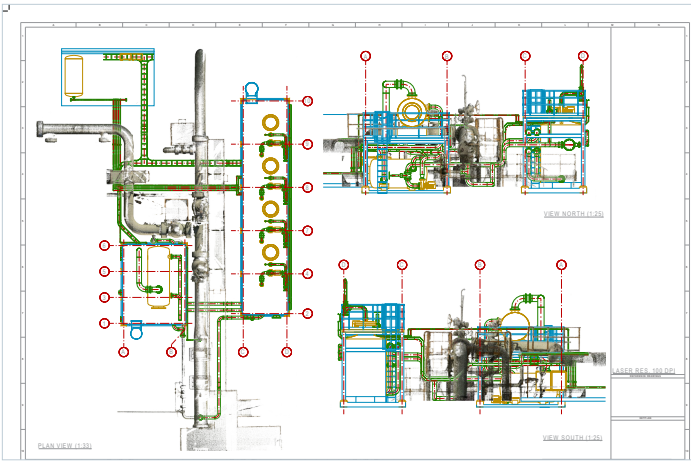
Layout and arrangement drawings can include laser data
